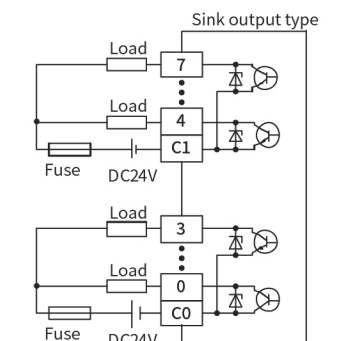
Figure 9 Transistor output equivalent circuit
