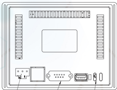
Power interface / COM communication port / HMI program download port
